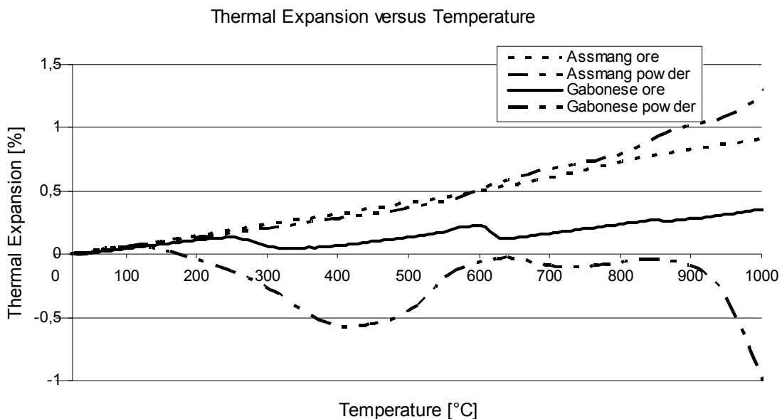
Figure 10: Thermal expansion in length of solid ore and powdered compacts
