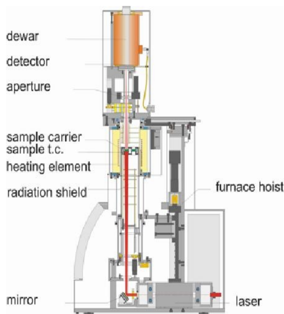
Figure 1: LFA 457 MicroFlash schema 4
