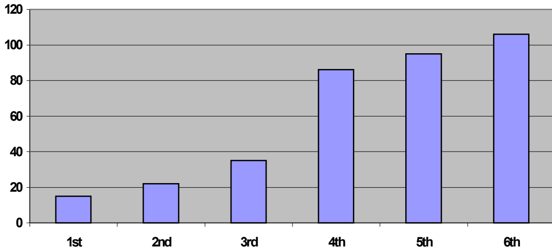
Figure 5: Flash Smelting Furnace campaign duration, months
