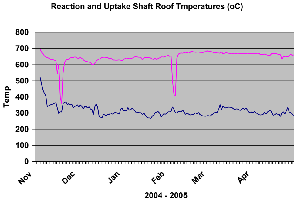
Figure 17: Flash Furnace roof temperature monitoring
