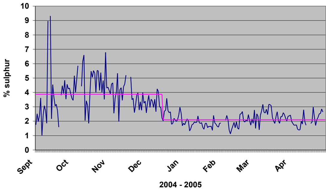
Figure 12: Sulphur levels in waste heat boiler dust
