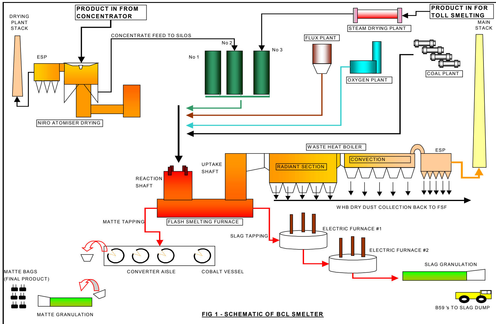
Figure 1: BCL Smelter Plant Flowsheet
