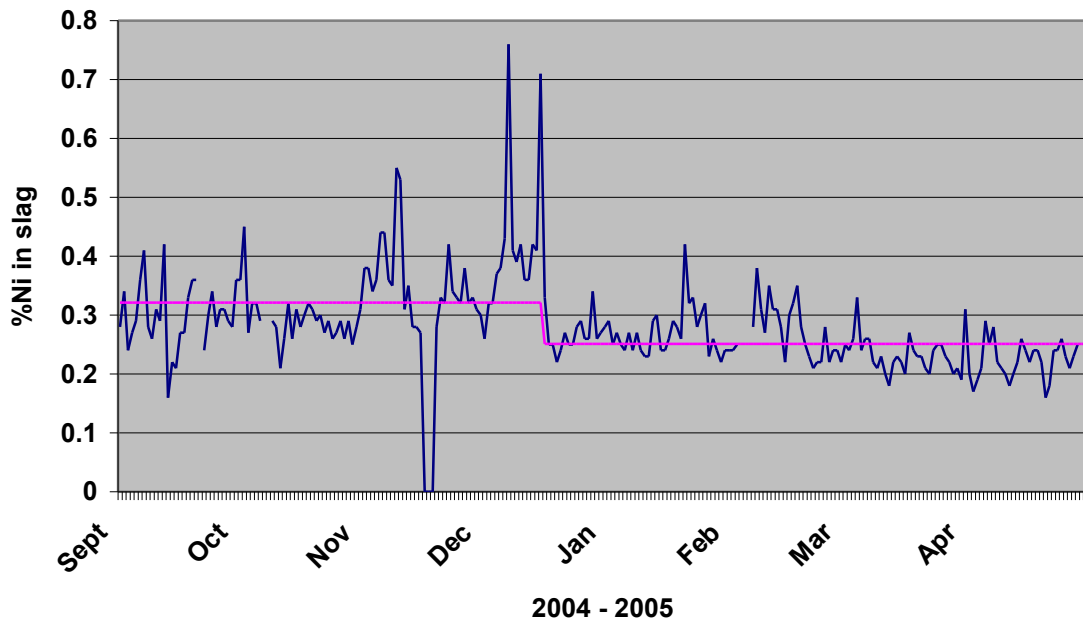
Figure 14: Nickel content of discard slag
