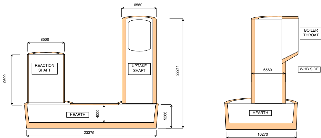
Figure 2: Dimensions of BCL Flash Smelting Furnace
