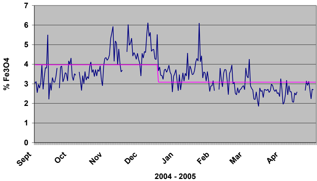
Figure 13: Magnetite levels in discard slag
