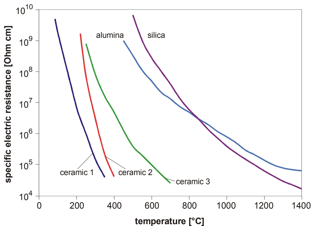
Figure 4: Relationship between temperature and the specific electrical resistance of various ceramic materials
