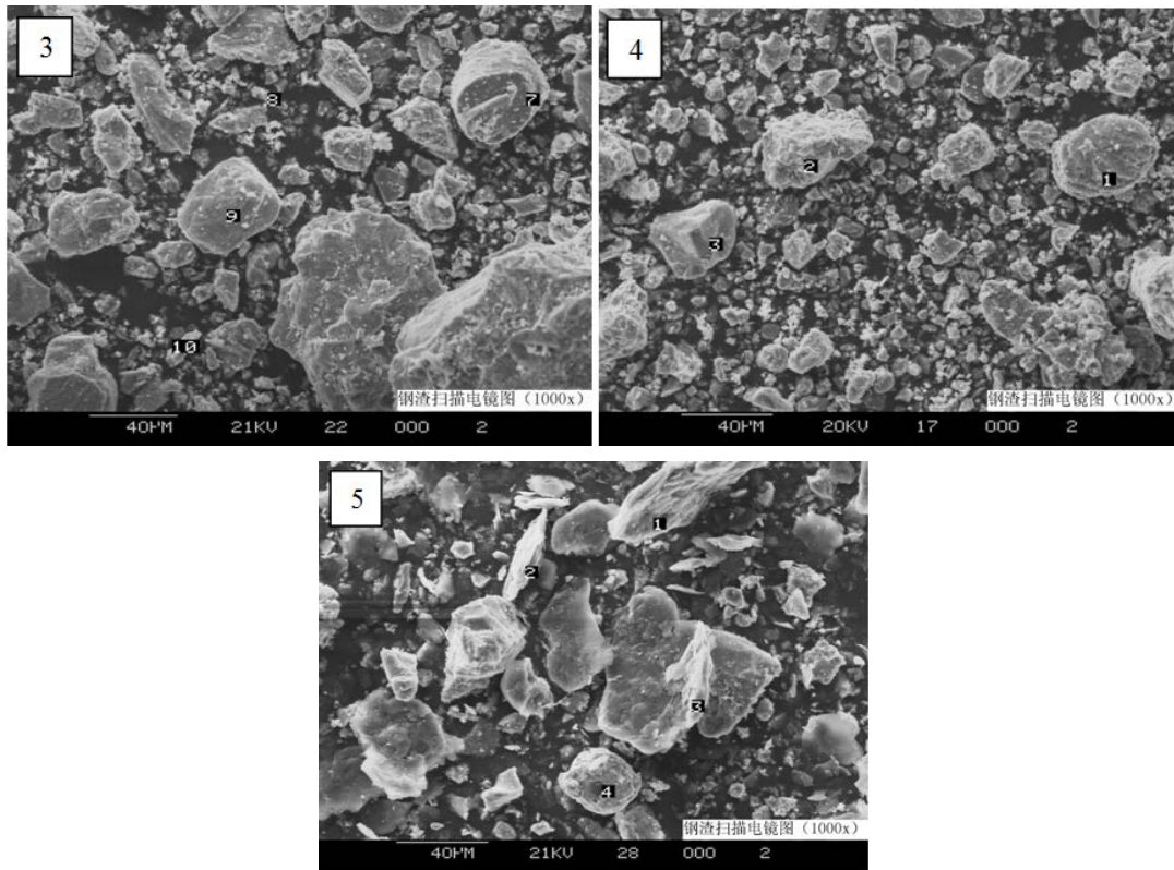
Fig. 1-5 Scanning Electron Microscope photos of converter steel slag (1000×)
