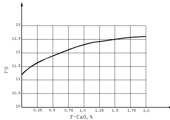
Fig.10 The relationship between content of f-CaO in steel slag powder and pH
