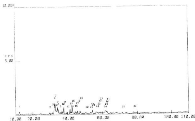
Fig. 6 X-ray Diffraction Patterns on Converter Steel Slag
