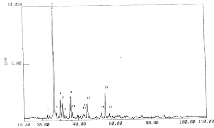
Fig. 7 X-ray Diffraction Patterns of Steel Slag
