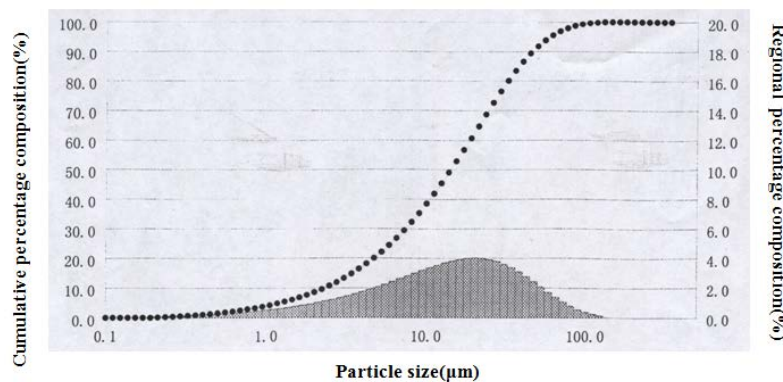
Fig.8 Distribution of grain size of converter steel slag powder (400m 2 /kg)
