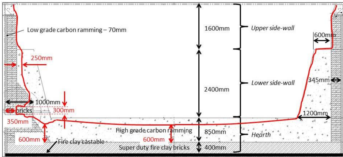
Fig. 1: Refractory wear profile (red line) of a 48 MVA SAF, used for SiMn production, excavated in 2013 in South Africa superimposed onto the refractory design drawing (black drawing).
