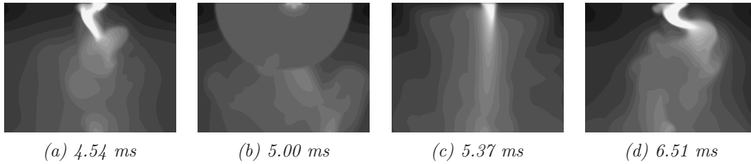
Figure 5. Model results for arc evolution as a result of low-temperature cathode fireball
