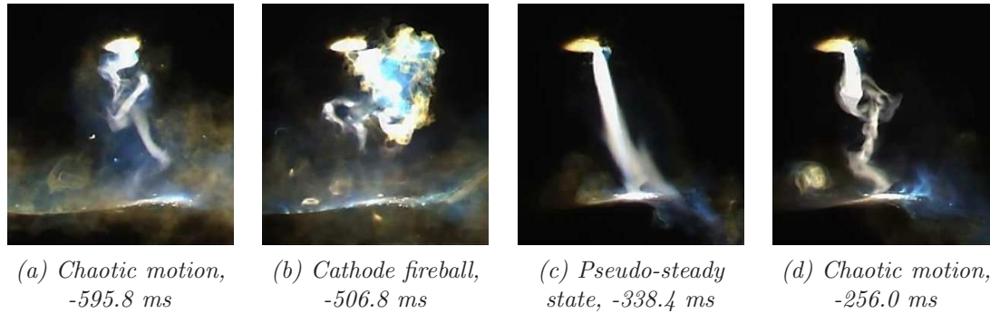
Figure 3. Sequence of frames from arc transition test at 3kA, showing various behavioural phenomena associated with arc extinction
