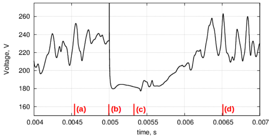
Figure 6. Measured voltage and current data for arc transition test (annotations refer to Fig. 5)
