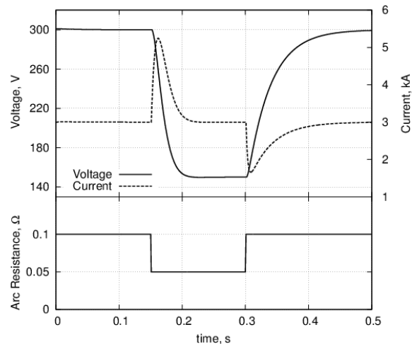
Figure 8. Circuit response to step change in R
