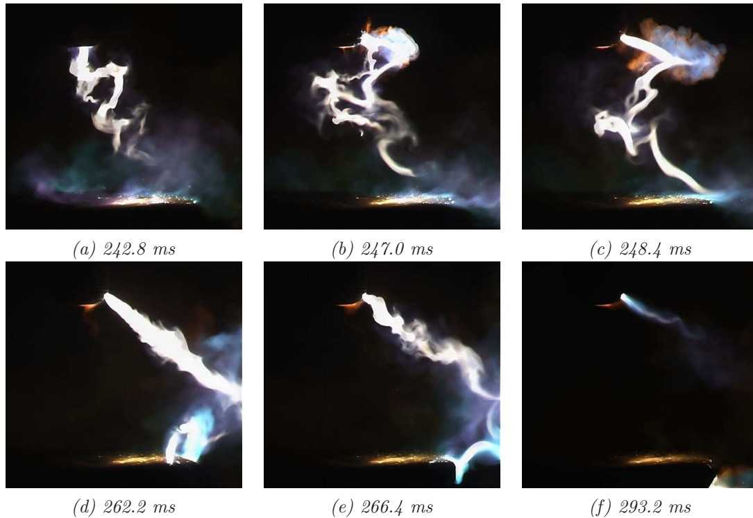
Figure 1. Sequence of frames from arc extinction test at 3kA, showing multiple transition events at different times
