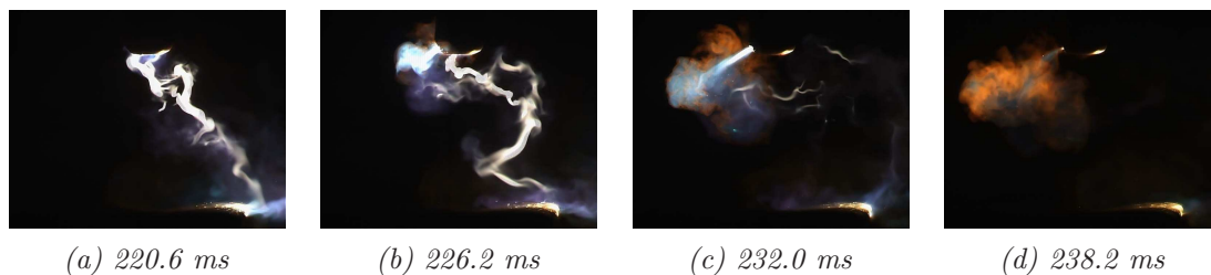
Figure 2. Sequence of frames from arc extinction test at 3kA, showing fireball event at different times
