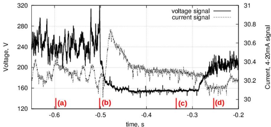
Figure 4. Measured voltage and current data for arc transition test (annotations refer to Fig. 3)
