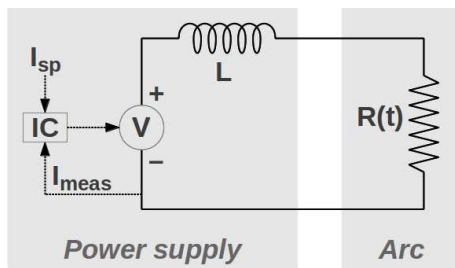
Figure 7. Simplified circuit diagram
