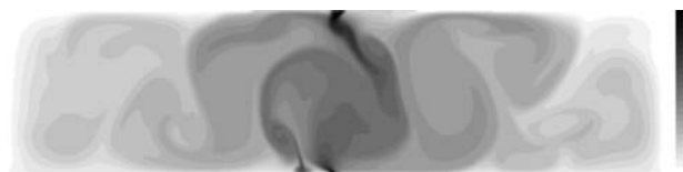
Figure 2—Temperature field at 9.98 ms
