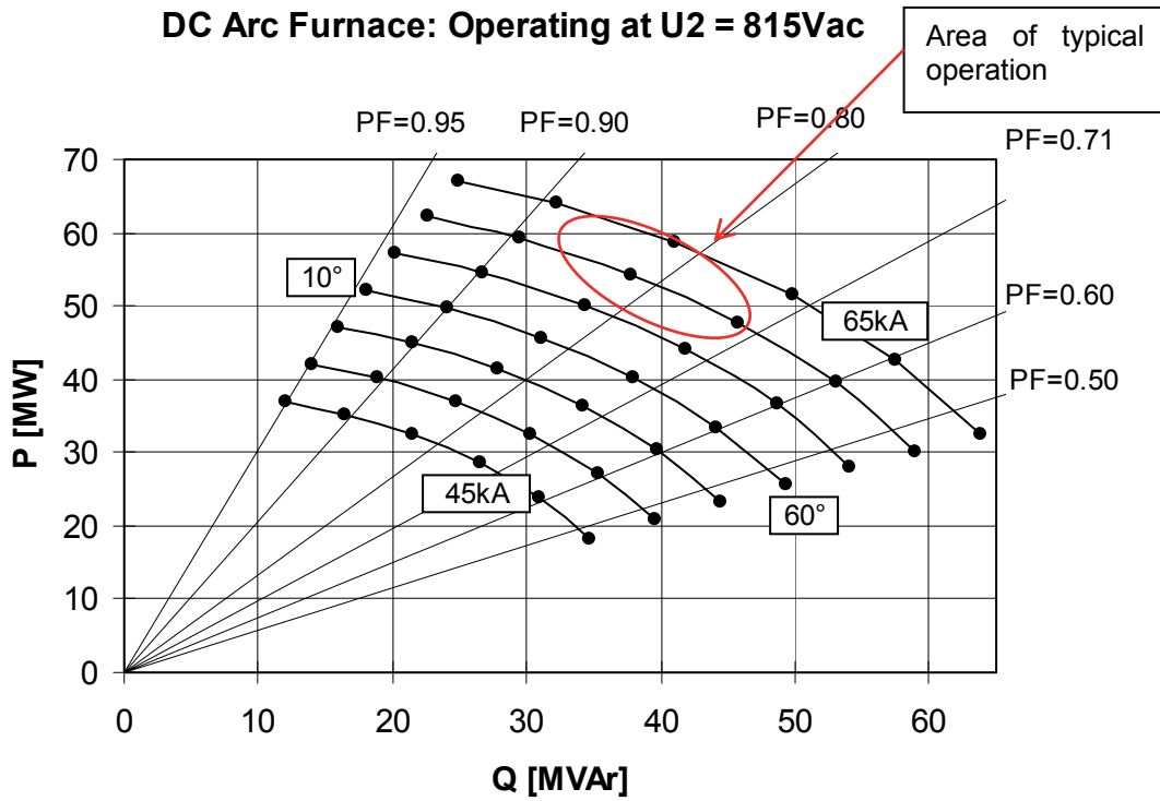
Figure 2: Sweeping on the curve of constant current (45 ... 65kA) at fix transformer secondary voltage: Resulting P [MW], Q [MVar] and power factor ( \cos \varphi ) can be taken out of the diagram
