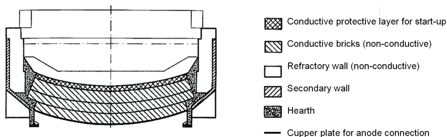
Figure 5: Principle sketch for conductive bottom electrode [2]
