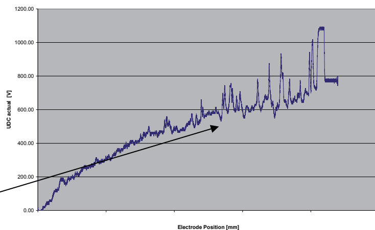
Figure 10: Shows the arc voltage in relation to the arc length at a constant current and fixed DC reactor impedance. It can clearly be seen that from a certain point onwards the voltage gets more and more unstable and finally the arc extinguishes completely.
