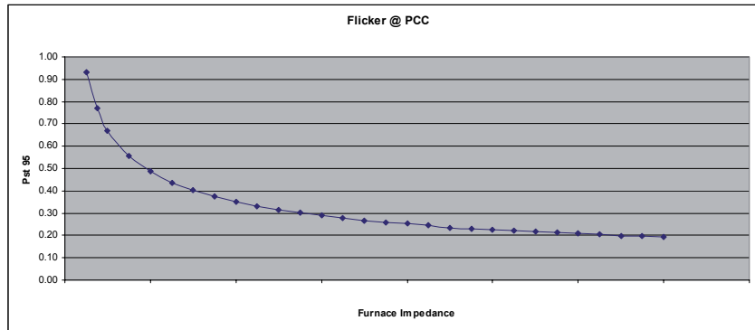
Figure 9: Shows the influence of the reactor sizing on the flicker level. The bigger the reactor's impedance, the lower the flicker. What can also be seen is that this effect saturates from a certain point onwards. When entering the saturation area, because of the higher losses, the weight and the cost of the DC reactor, it is not economically viable anymore to further increase the reactor size. Should a further flicker level reduction still be required, an SVC needs to be installed. - In MFC's case, the reactor size is far away from this saturation area.
