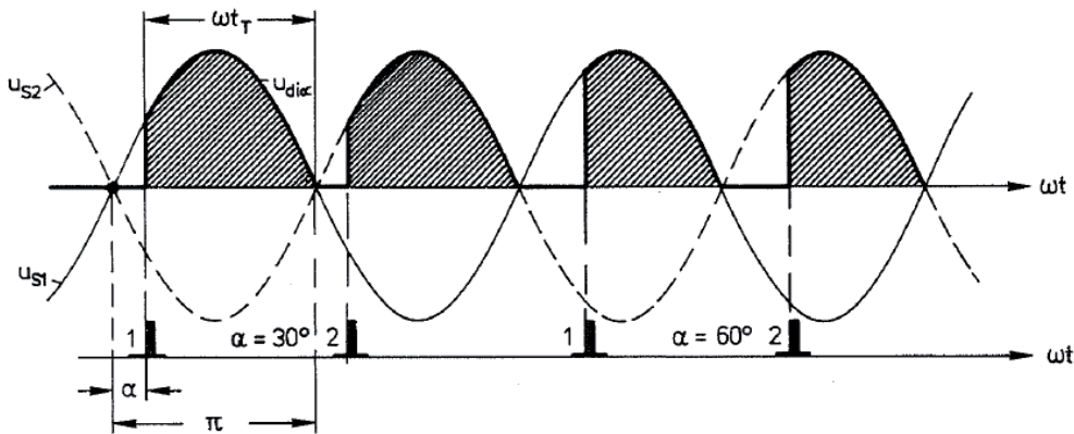
Figure 3: The bigger the firing angle \alpha , the lower is the rectifier's voltage and DC current. Also, the higher the firing angle, the higher is the phase shift between voltage and current on the AC side, resulting in higher reactive power and hence a lower power factor \cos \varphi (= active power [P] divided by apparent power [S]).
