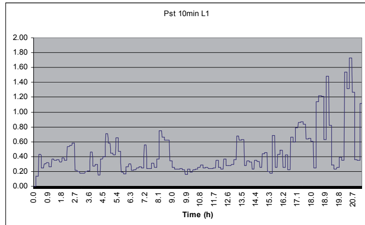
Figure 8: Actual flicker measurements taken on the 33kV bus with the furnace running at full load (60 MW)
