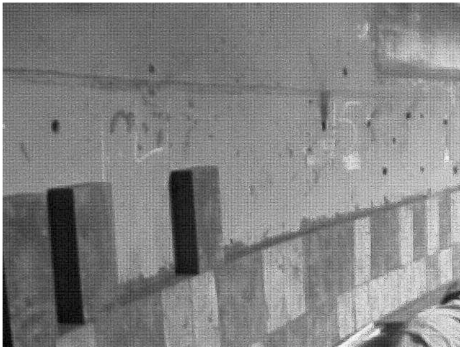
Figure 1. M12 lining – graphite tiles installation.
