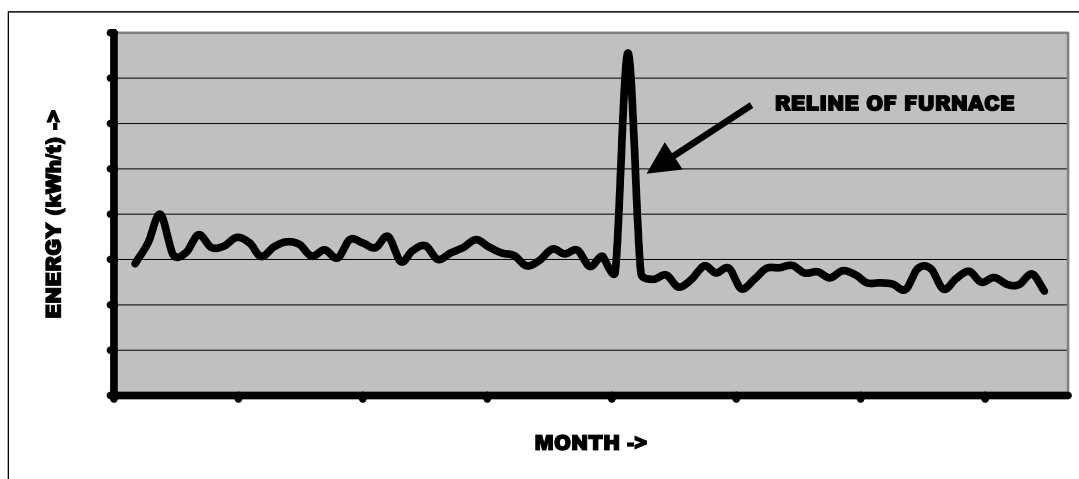
Figure 4. Specific energy consumption for the production of HCFeMn on M12.
