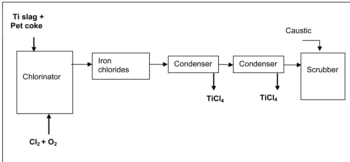
Figure 2: Process flow diagram for TiCl 4 production at Mintek pilot plant
