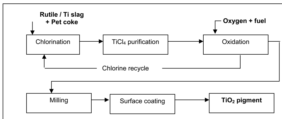
Figure 1b: TiO 2 manufacturing by Chloride process
