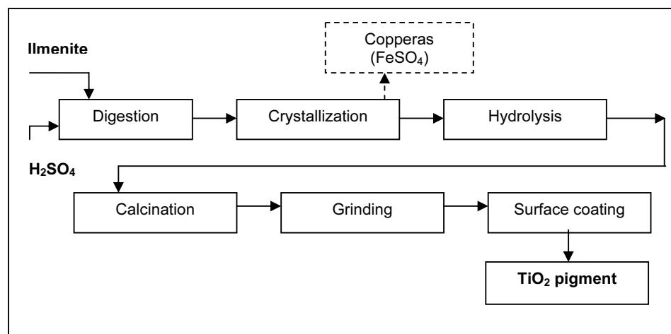
Figure 1a: \text{TiO}_2 manufacturing by Sulphate process
